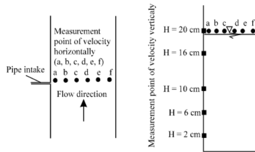
Fig. 5: Location of velocity measurement
