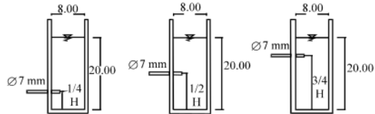
Fig 3: Research flume
