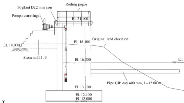
Fig. 1: An illustration of a free intake structure
