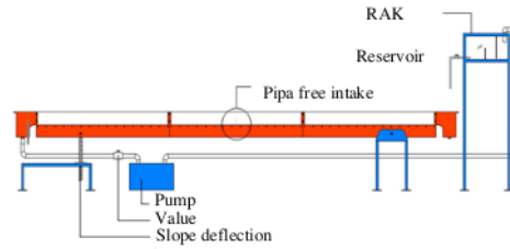
Fig 3: Research flume
