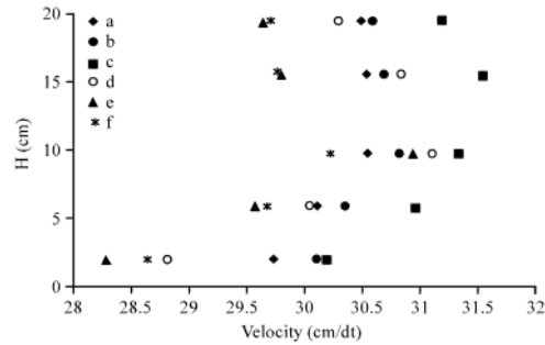
Fig. 7: Distribution of velocity with free intake structures
